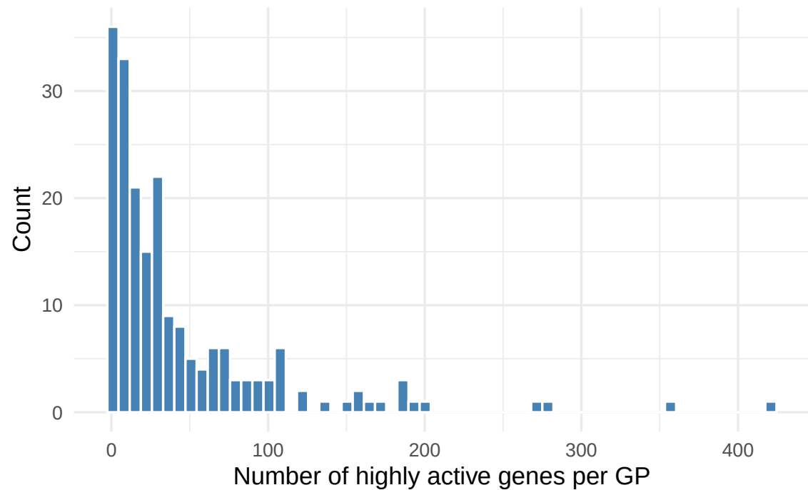
Histogram of highly active genes per GP
